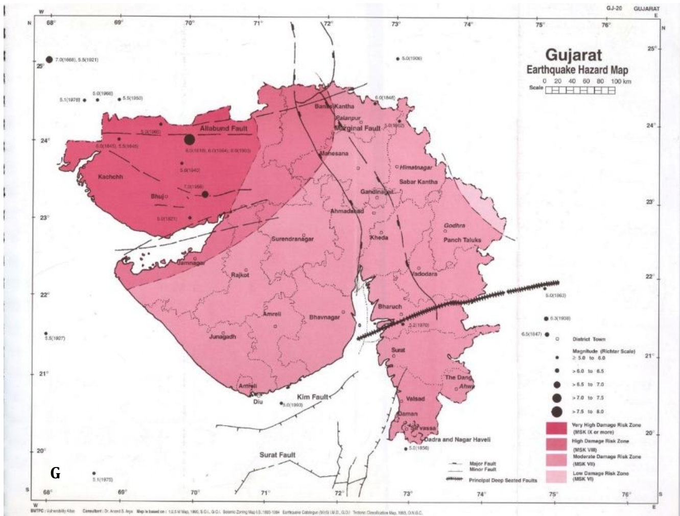
Figure 2. Zoomed Gujarat portion of the Seismic Zoning Map of India which also corresponds to realistic Intensity distribution during Bhuj 2001 earthquake . Locations of some past earthquakes are shown.
